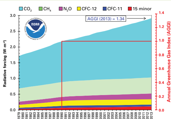
Figure 1. Atmospheric radiative forcing, relative to 1750, of LLGHGs and the 2013 update of the NOAA Annual Greenhouse Gas Index (AGGI)
