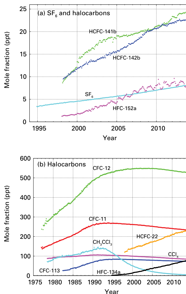
Figure 7. Monthly mean mole fractions of sulphur hexafluoride ( \text{SF}_6 ) and a suite of halocompounds ( \text{SF}_6 and minor halocarbons (a) and major halocarbons (b)). The numbers of stations used for the global analyses are as follows: \text{SF}_6 (23), CFC-11 (24), CFC-12 (25), CFC-113 (23), \text{CCl}_4 (21), \text{CH}_3\text{CCl}_3 (23), HCFC-141b (9), HCFC-142b (13), HCFC-22 (13), HFC-134a (9) and HFC-152a (8).
