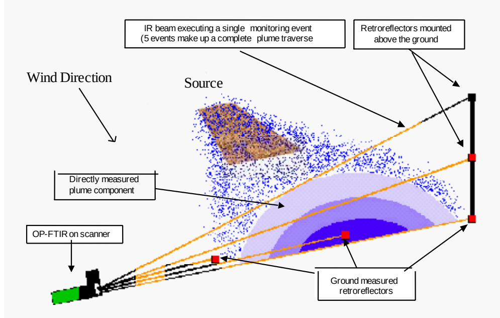
Figure 2-2. Example of a plume's characterization and emission calculation under a crosswind using the PI-ORS method.
