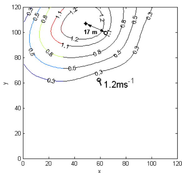
Figure 7-4: Plume source location using ORS method by horizontal scanning
