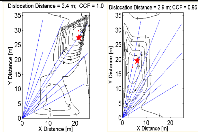
Figure 2-1. Examples of experimental ethylene source localization using OP-FTIR scanning in the radial configuration.
