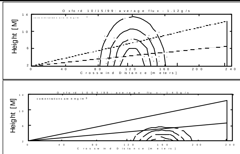
Figure 2-3. Examples of emission calculations for a controlled release under stable and unstable atmospheric conditions, respectively
