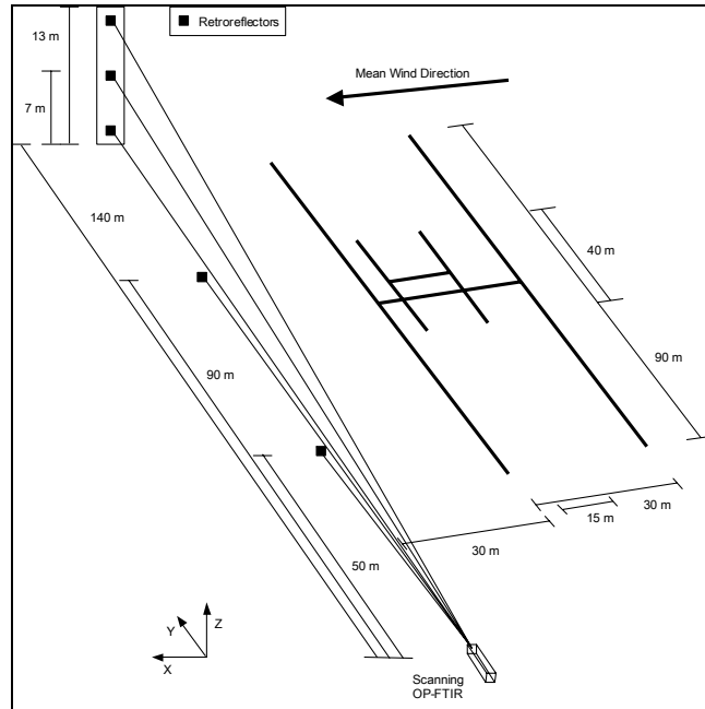
Figure 3-3: Configuration for crosswind plume measurement
